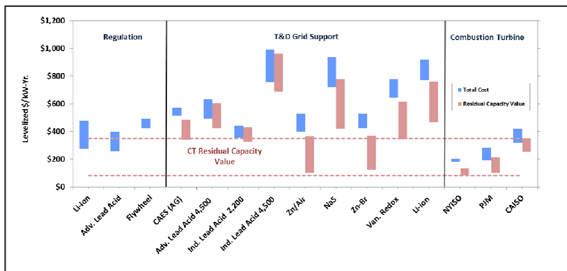
Figure ES-16 Levelized Total and Residual Capacity Cost for Storage Technologies Compared to Combustion Turbine
