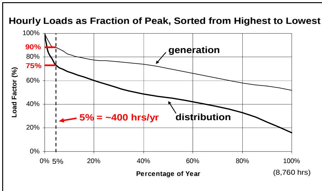
Figure 3-7 Significant Industry Investments in T&D Infrastructure are Required for Only Approximately 400 Hours per Year
