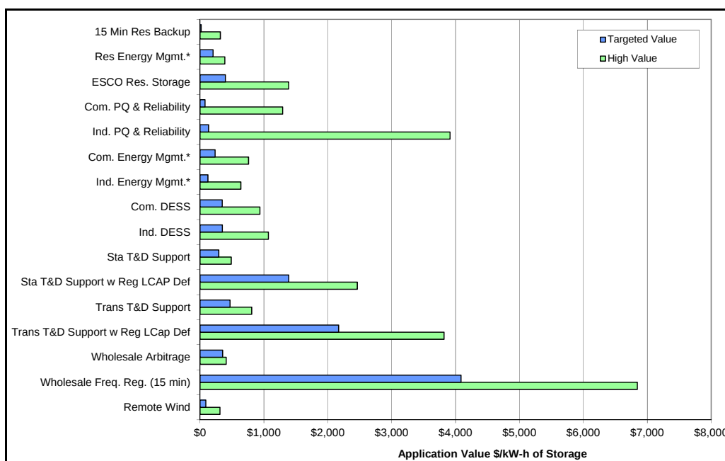
Figure ES-11 Summary of Target and High Application PVs for Energy Storage
